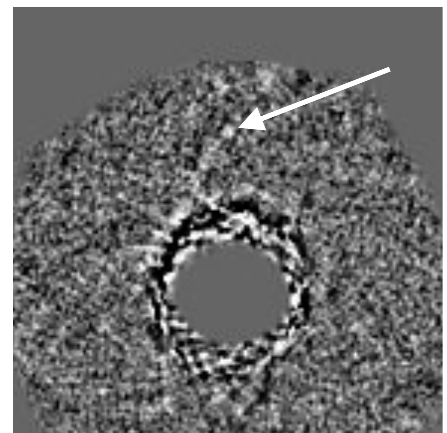
Fig. 5: Planet #2, with a differential magnitude (dmag) of 17, is successfully detected by K-Stacker using the Reduced images displayed in Figure 3.
