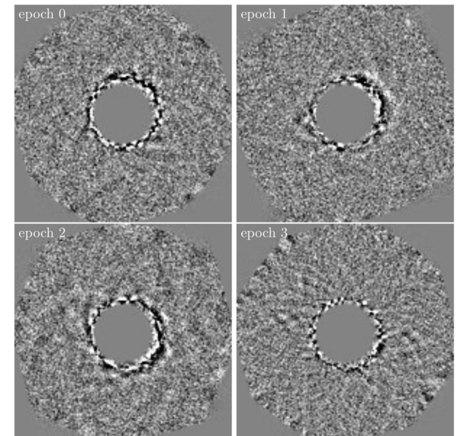
Fig. 3: Reduced PCA-ASDI observations with VIP, wherein planet #2, with dmag=17, remains undetected in individual epochs.
